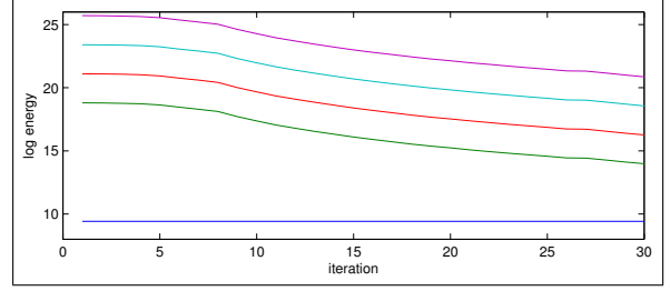
Figure 2. Convergence of the obtained primal feasible solution for four datasets which differ only by the values used as “infinity”. The energy values are plotted in logarithmic scale. From bottom to top: optimal log-energy, primal bounds corresponding to infinity values equal to 10 000, 100 000, 1 000 000 and 10 000 000.
